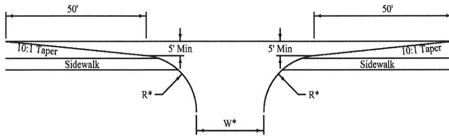
Figure 5L-4.03: Offset Radius and Driveway Tapers
